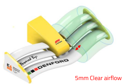
Multi Vane
